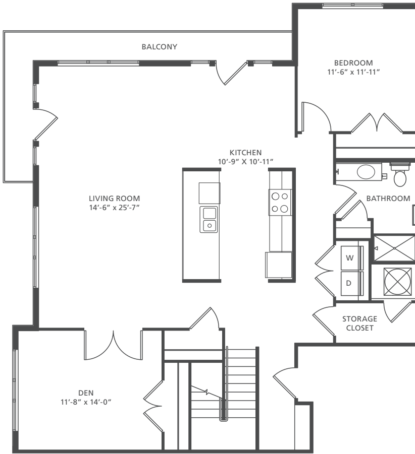
MAIN LEVEL
